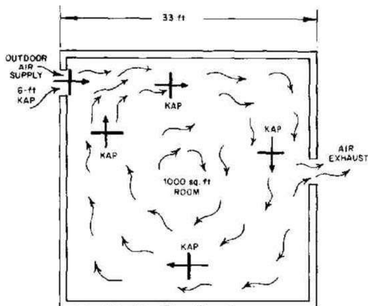
Fig. 16. The use of air-distribution KAPs.
