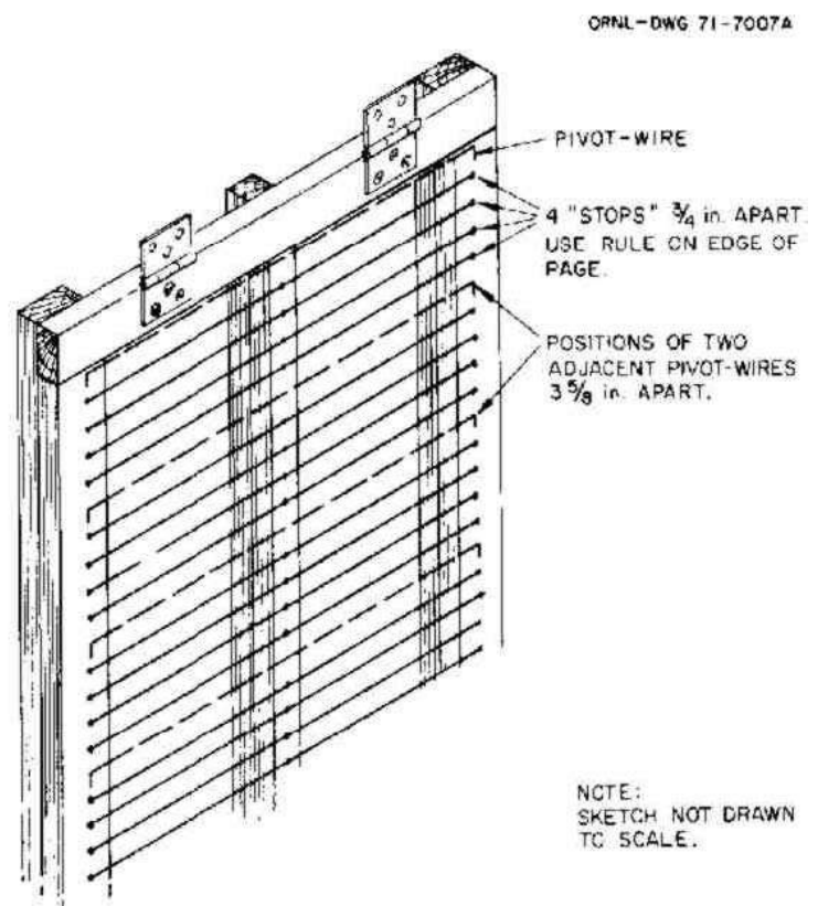
Fig. 11. Positions of pivot-wires and flap-stops.
