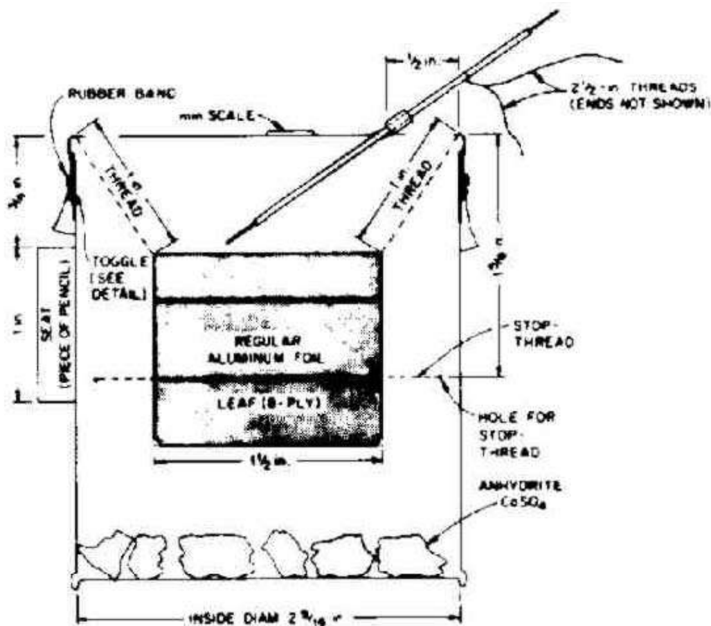
Fig. 229a (Charging a KFM)
