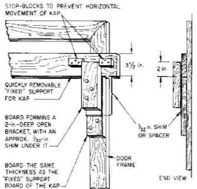
Fig. 19. Quick-removal bracket for KAP. ORNL DWG 72-6365A
