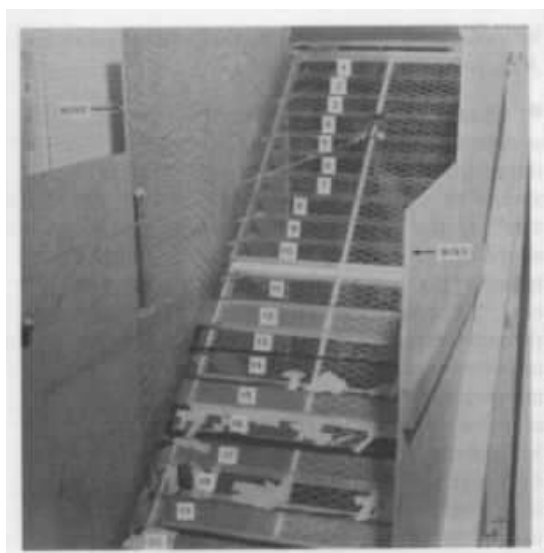
(Photograph) Fig. 6.1. A 6 foot KAP tested for durability at Oak Ridge. After 1000 hours of operation during which it pumped air through a room at a rate of 4000 cubic feet per minute (4000 cfm), there were only minor tears in the plastic flaps.
