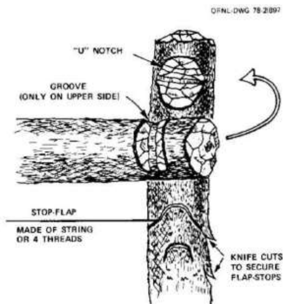
Fig. 21. Sticks ready to be tied together to make a KAP frame. ORNL-DWG 78-21897
