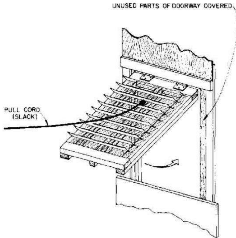
Fig. 1. Section through the upper part of a doorway, showing operation of a KAP. (ORNL-DWG 66-12320A)
