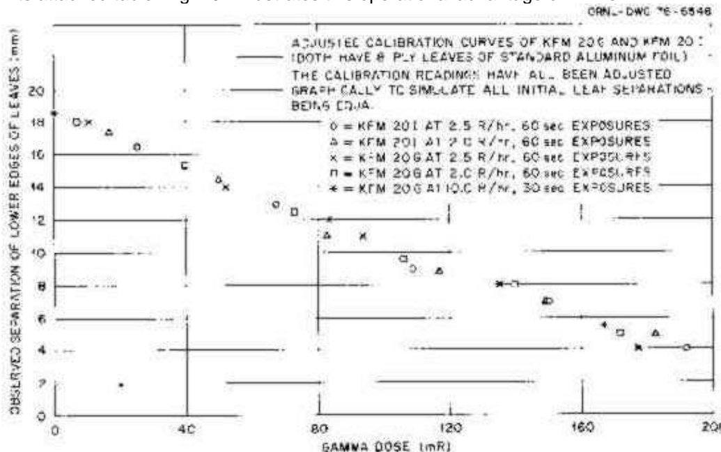
Fig. 10.2 Normalized Calibration Points for Two KFMs, Showing the Straight-Line Relationship Between Milli-roentgen Radiation DOSES and Resultant Readings. The complete instructions for making and using a KFM (see Appendix C) explain how an operator with a watch can use this instrument to accurately measure DOSE RATES. (Text in Graph) ADJUSTED CALIBRATION CURVES OF KFM 20 G AND KFM 20 I (BOTH HAVE 8-PLY LEAVES OF STANDARD ALUMINUM FOIL) THE CALIBRATION READINGS HAVE ALL BEEN ADJUSTED GRAPHICALLY TO SIMULATE ALL INITIAL LEAF SEPARATIONS BEING EQUAL. ORNL-DWG 76-6548
