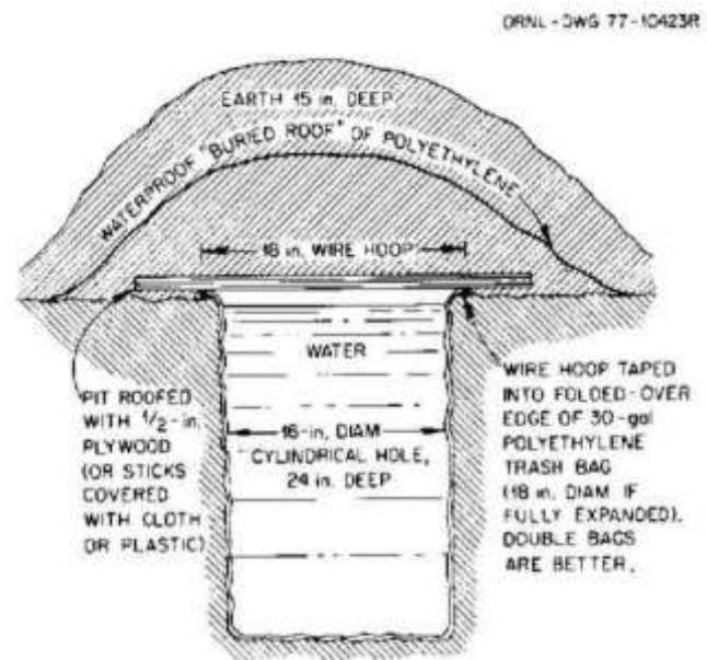
Fig. 8.3. Vertical section of cylindrical water storage pit lined with two 30-gallon waterproof plastic bags. This pit held about 20 gallons.
