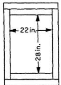
Fig. Pg. 252 A vertical blast -protective entry. 22 in. x 28 in.
