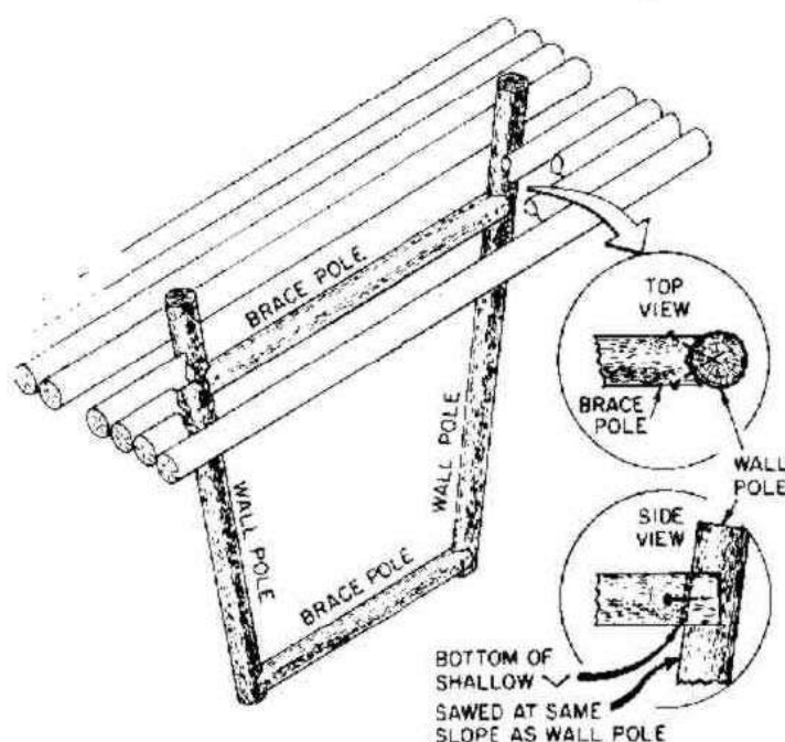
Fig. D.7. An illustration of several ways to shore a trench in unstable earth, using various materials. A 4-piece frame (consisting of 4 poles, or 4 boards, installed as shown above) should be installed every 2-1/2 feet along the length of the trench, including the horizontal parts of the entryways. All parts of the shoring should be at least 2 inches below the roof poles, so that the downward forces on the roof will press only on the earth. (ORNL-DWG 78-14430R)
