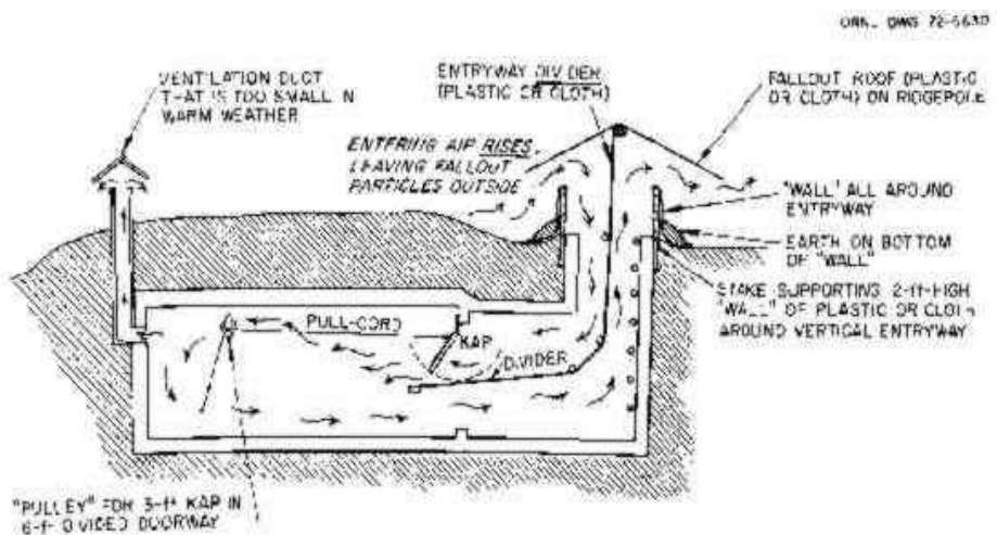
Fig. 15. Ventilating a shelter when the air-exhaust opening is too small. ORNL DWG 72-6630
