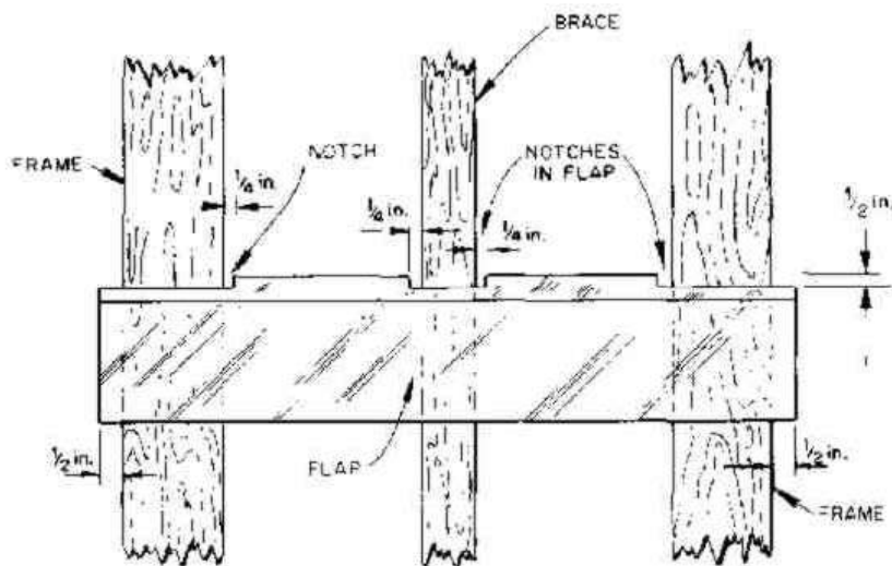
Fig. 6. Sizes of notches in flaps.
