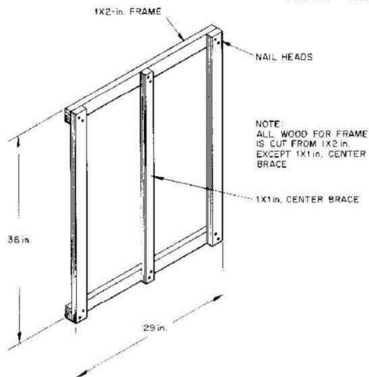
Fig. 3. KAP frame (looking at the back side of the frame). ORNL 71-7003
