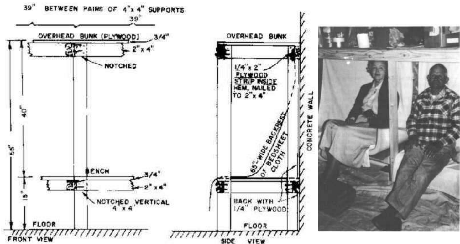
Fig. 17.5. Backrests of Bedsheet Cloth and 2-Inch-Thick Pads Make Sitting and Sleeping Comfortable.
