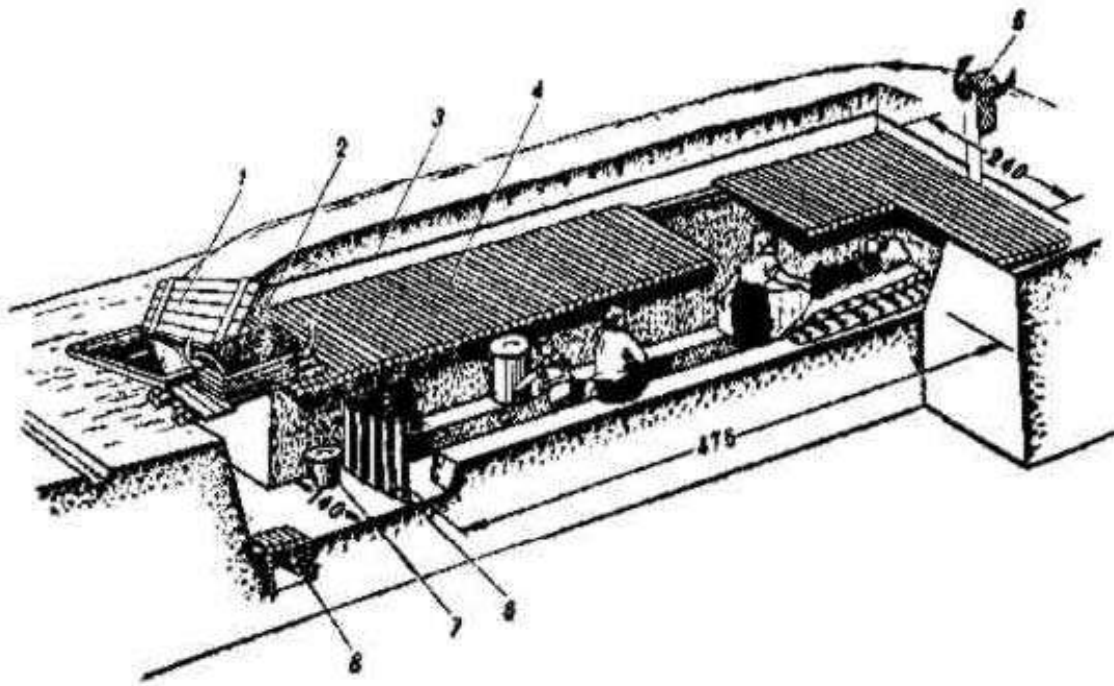
(Illustration) Fig. 6.5. [Figure 20.] Wood-Earth Shelter without Lining of the Walls for Clay Soils, 10 Occupants: 1 - Trap Door; 2 - Dust Filter with a Straw Packing (hay); 3 - Earth Cover 60-80 cm thick; 4 - Roofing made of Poles; 5-Exhaust Duct with Damper; 6 - Curtain made of Tightly Woven Cloth; 7 - Removable Container for Wastes; 8- Water Collecting Sump.
