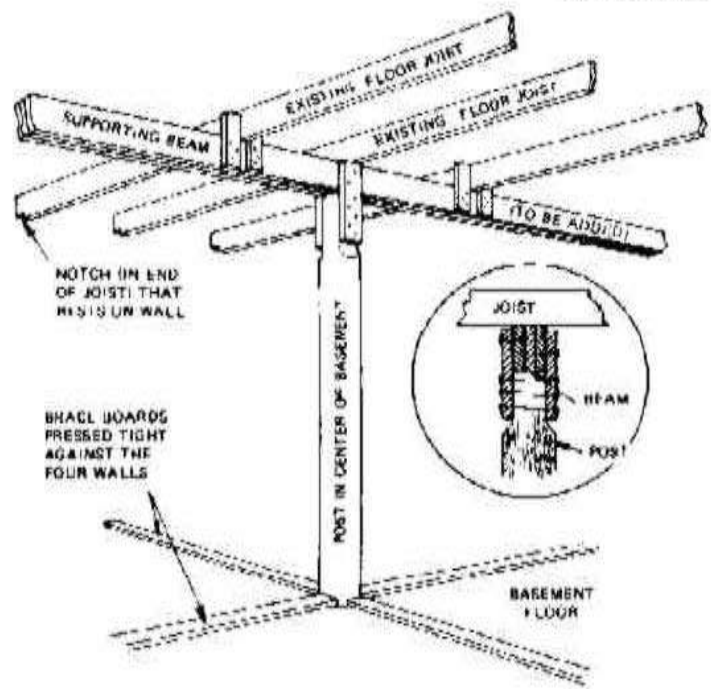
Fig. 5.8. Supporting beam and one of its posts installed to increase the load of shielding material that can be carried safely by the floor above a home basement.
