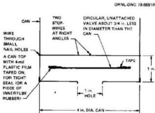
Fig. 8.10. Lower part of an expedient bail-can. The unattached, "caged" valve can be made of a material that does not have the springiness of soft rubber.
