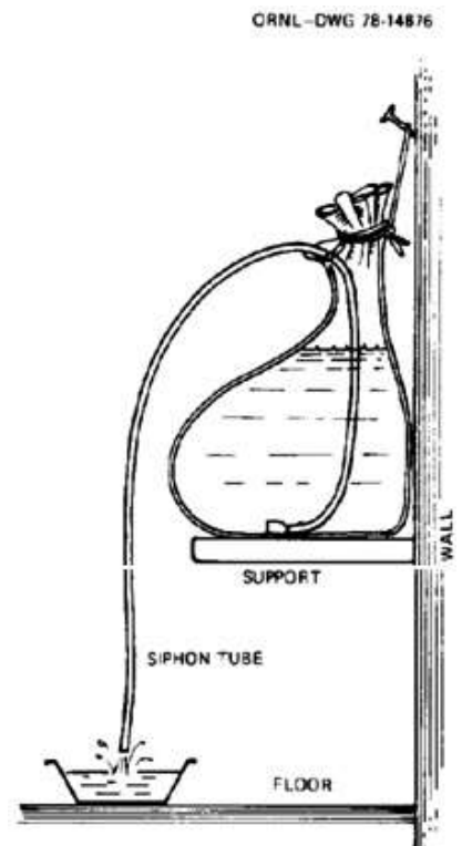
Fig. 8.7. Water siphoned into a belowground shelter.
