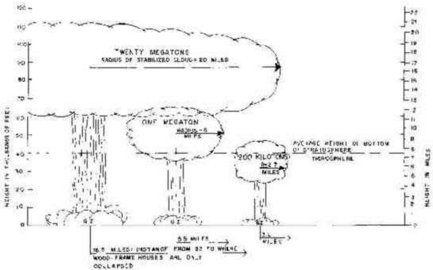
Fig. 4.1. Stabilized radioactive fallout clouds shown a few minutes after air-burst explosions, with distances from Ground Zeros at which the wood frames of typical homes are almost completely collapsed. The clouds from surface or near-surface bursts are almost as large, but the distances of blast damage are reduced by around 38 percent.
