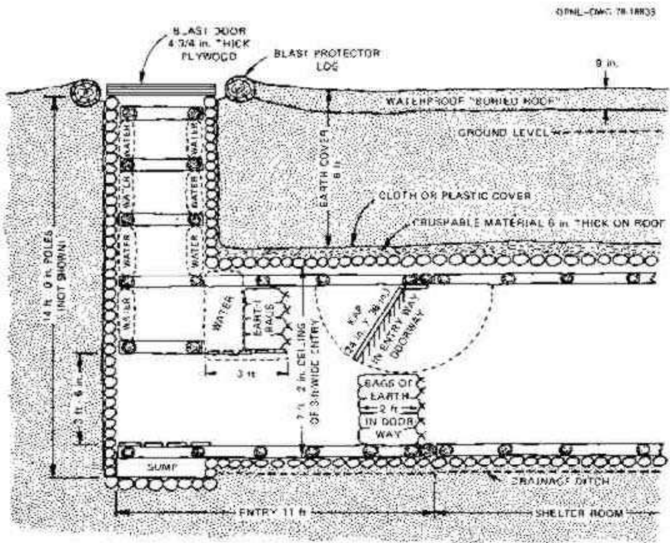
Fig. D.20. Entryway of Small-Pole Blast Shelter shielded against initial nuclear radiation. This sketch is a simplified vertical section through the centerline of one end of the shelter. ORNL-DWG 78-18835
