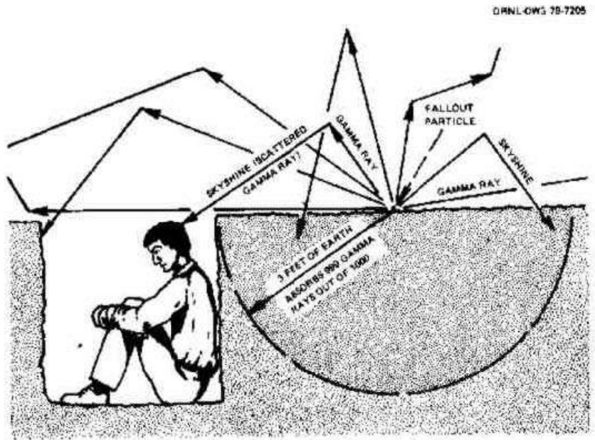
Fig. 5.3. Simplified illustration of barrier shielding and skyshine (scattered gamma radiation). An open trench provides poor protection. ORNL.DWG 78.7205
