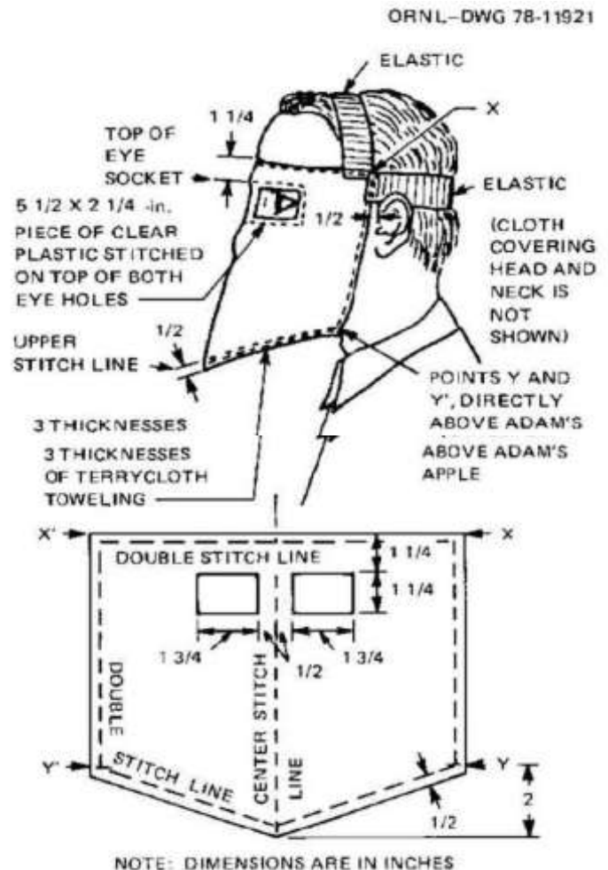
Fig. 15.9. A Russian-type homemade fallout mask. For most Americans this will continue to be a low-priority item as long as Russian warheads are large. ORNL-DWG 78-11921
