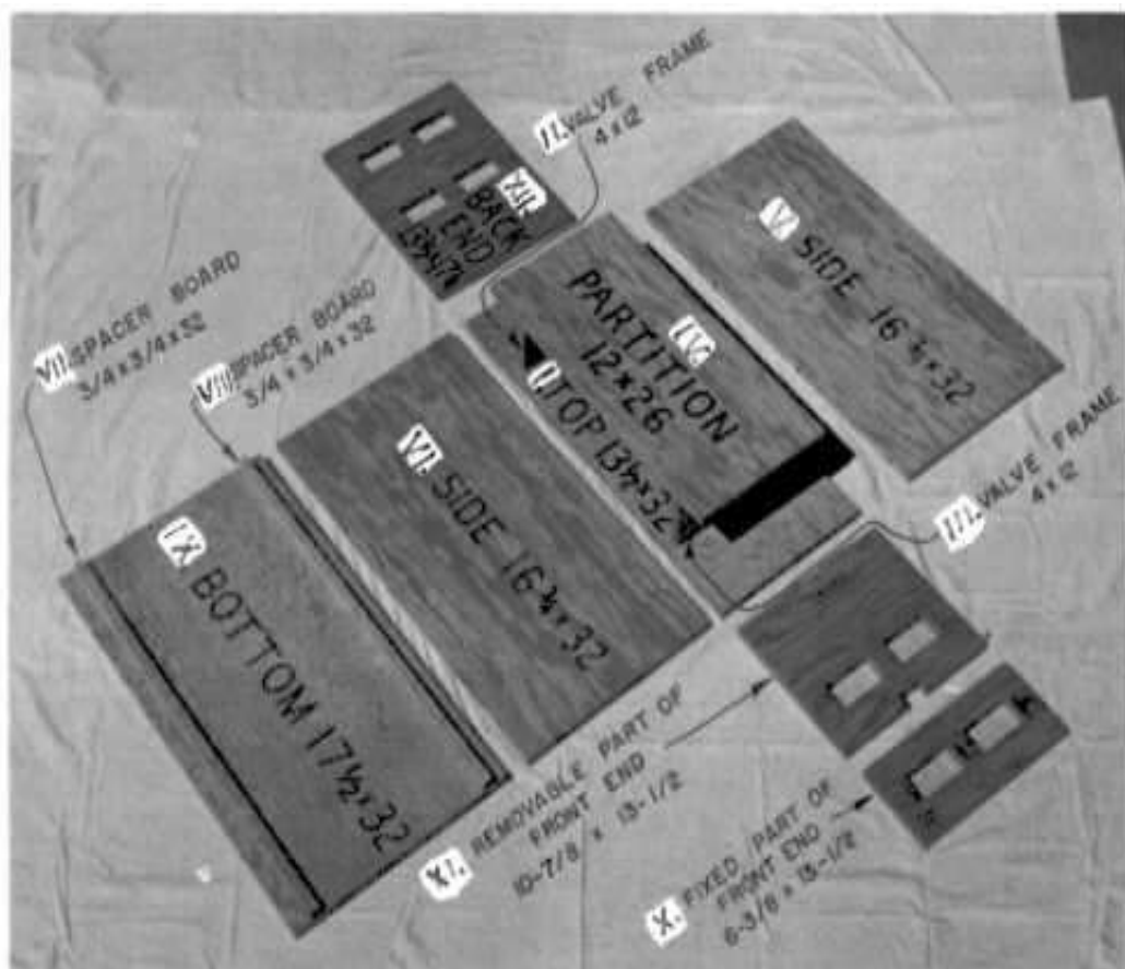
Fig. 12. Parts of the Pump "Box", with Dimensions in Inches. The Roman numbers give the best tested order for attaching these parts to each other.
