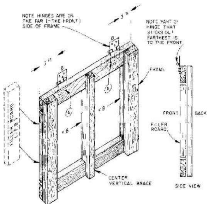
Fig. 4. Completing the frame. ORNL- DWG 66-12322A
