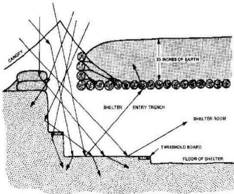
Fig. 5.5. Skyshine coming into a shelter through a vertical entry would be mostly absorbed while turning into and traveling down the entryway trench. ORNL-DWG 78-7204
