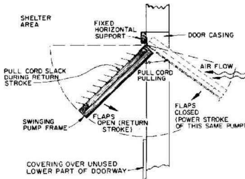
Fig. 2. KAP in doorway (with flaps open during its return stroke). (ORNL-DWG 66-12319A)
