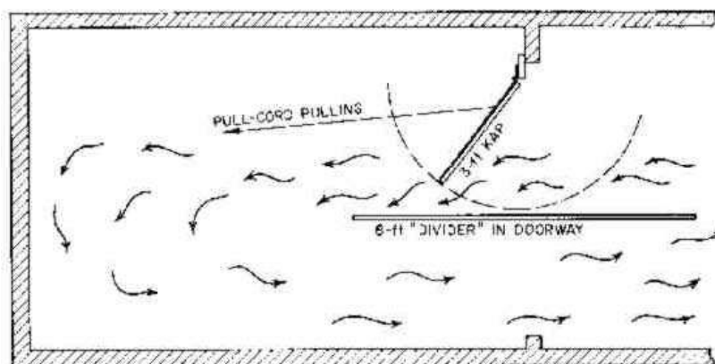
Fig. 27. Use of a "divider" to ventilate a shelter with only one opening. ORNL DWG 75-8203
