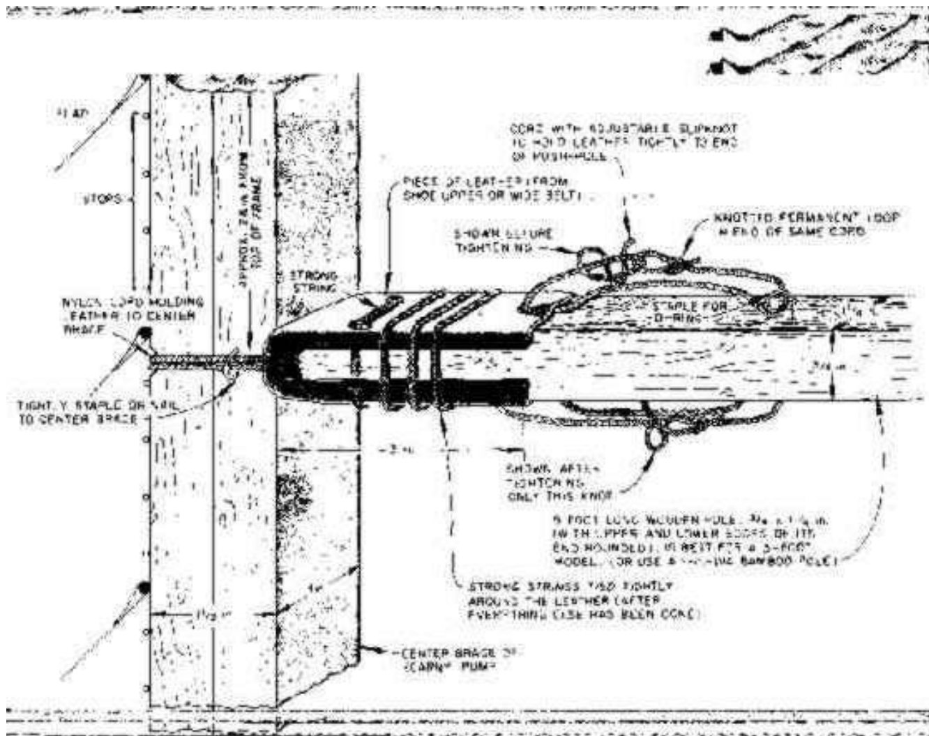
Fig. 26. Push-pole flexible connection. ORNL DWG 66-12332R
