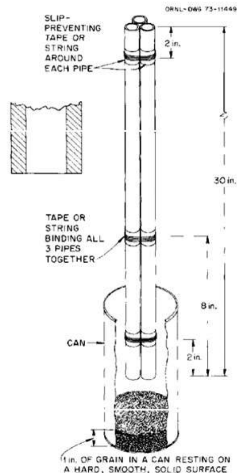
Fig.9.1. Improvised grain mill
