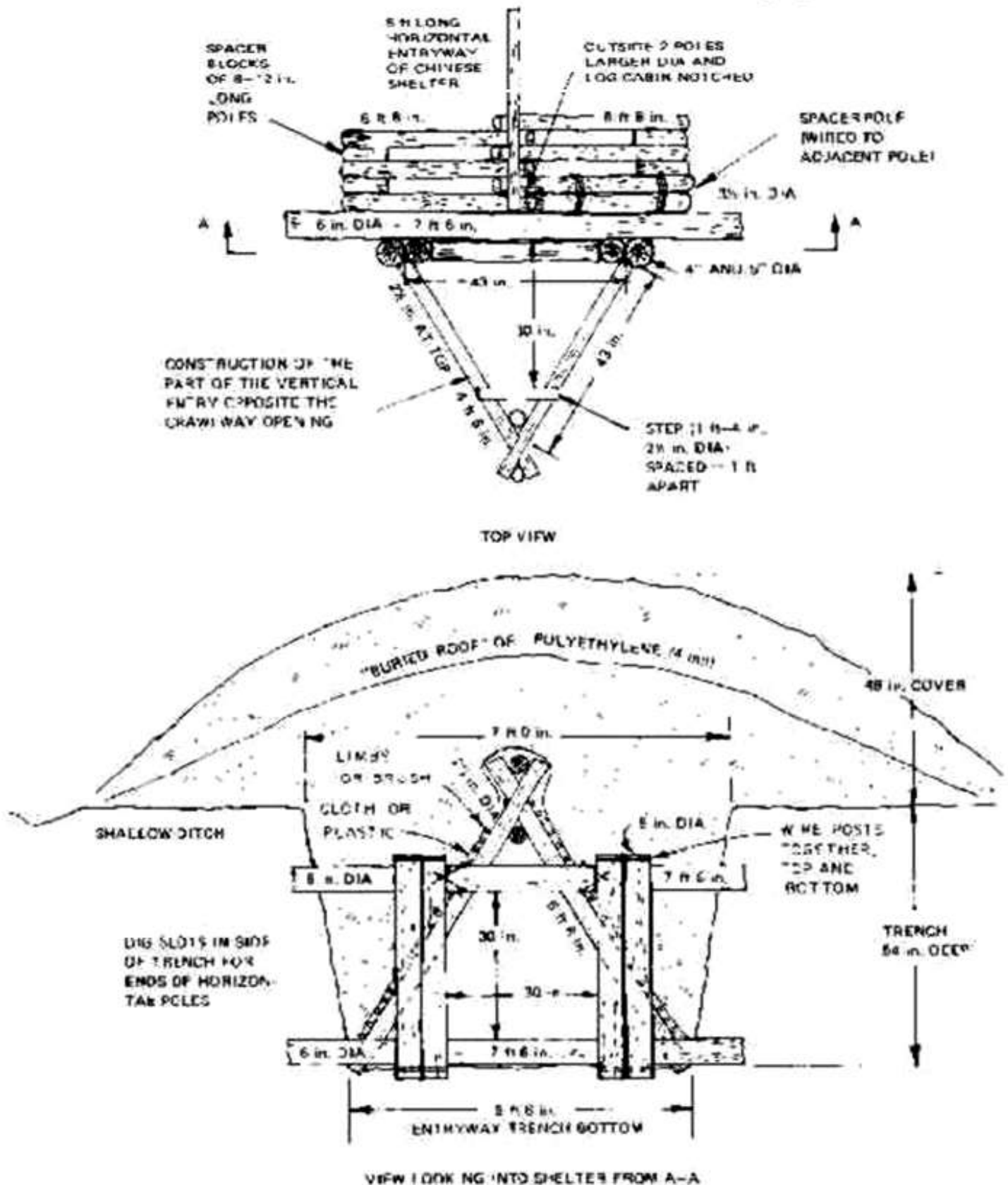
Fig. D. 11. Lower part of a vertical triangular entry, showing its connection to the horizontal part of the shelter entry. (ORNL-DWG 78-14675)
